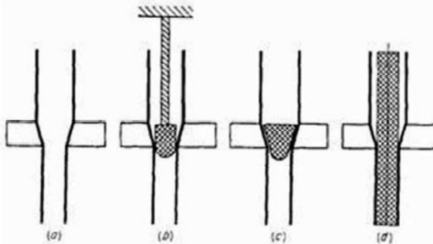
Tube drawing process by (a) Sinking (b) Fixed plug (c) Floating plug (d) Moving mandrel
